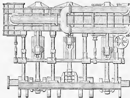
ENGINE OF STEAM YACHT ONEONTA.
